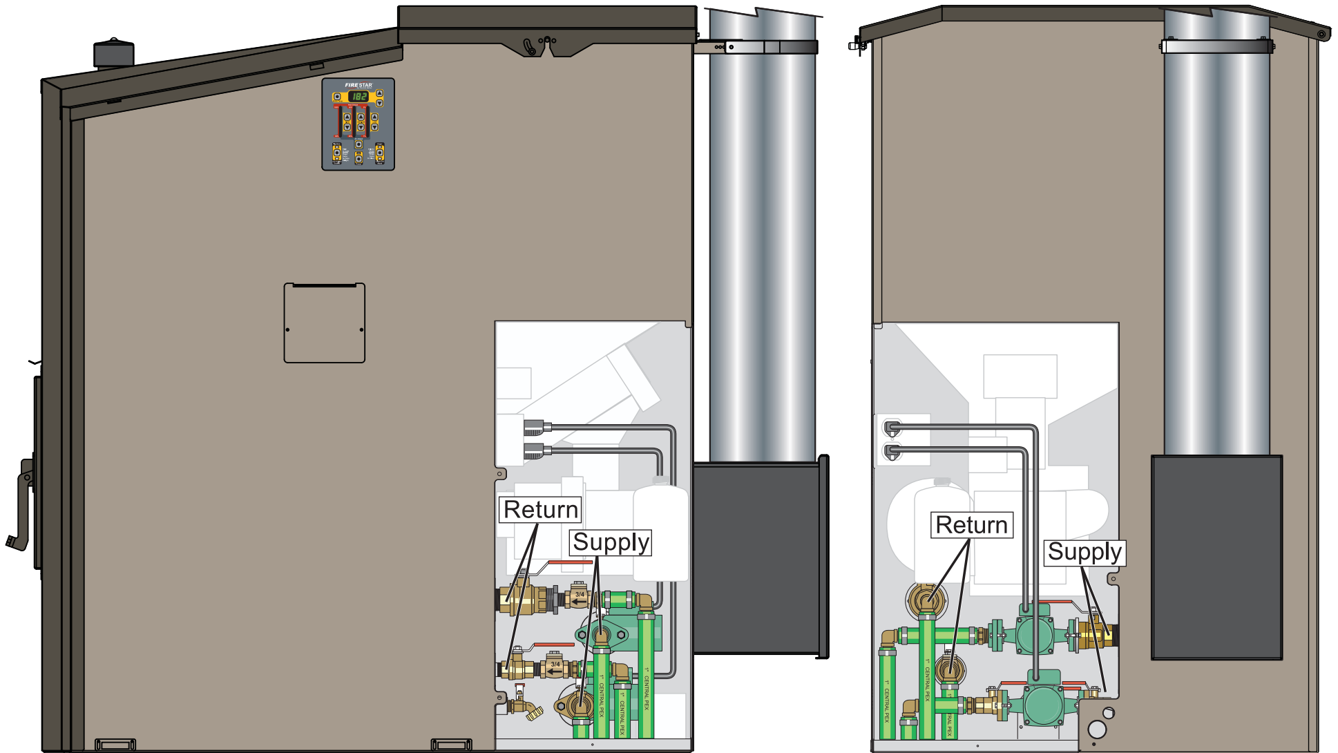
Side View
